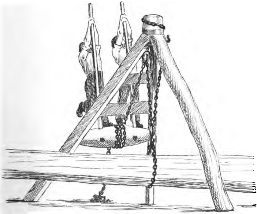
Fig. 295.—Derrick for raising logs on to carts. ( Vide p. 313.)
